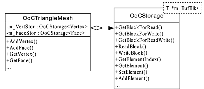
Fig. 6. Out-of-core storage.
